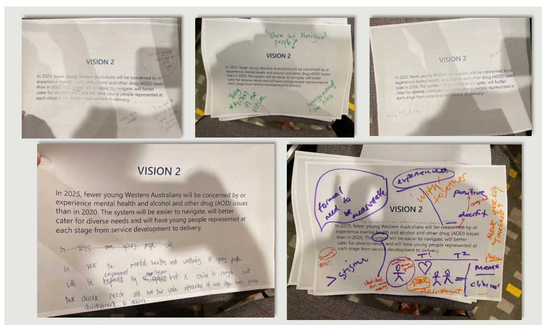
Figure 4 | Example comments
